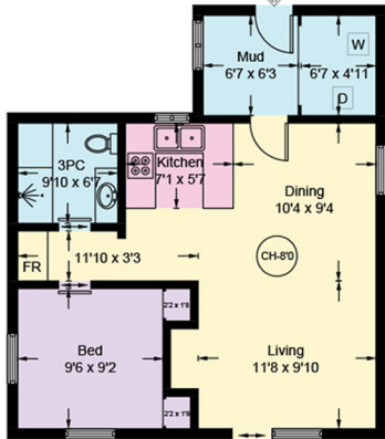
Main Floor (Cabin) - 617 sq ft
